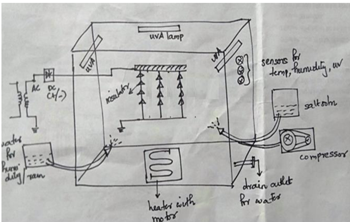
Figure 2: Representative model of variable stress ageing chamber
